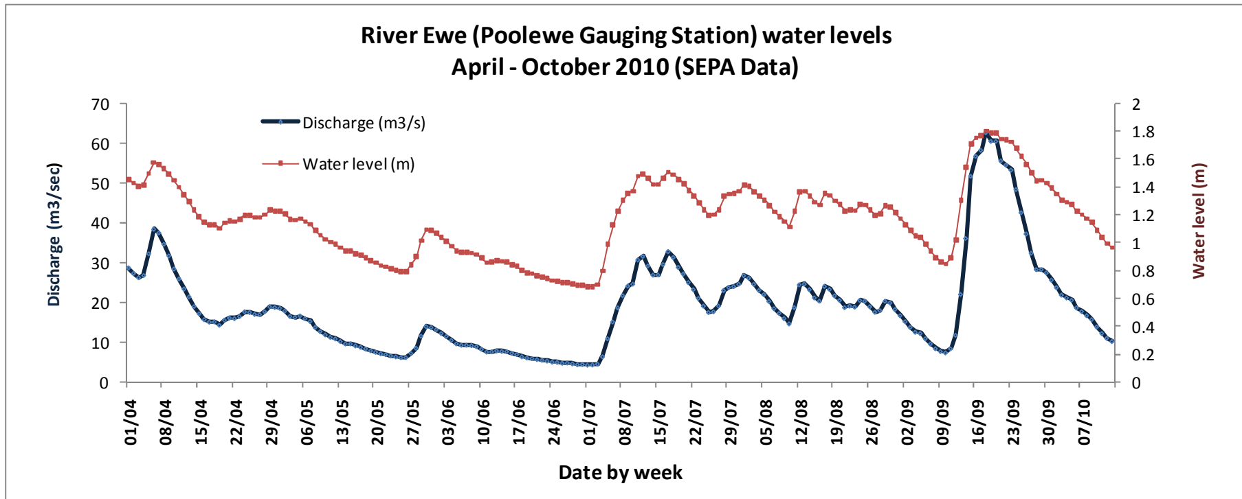
River Ewe water levels and discharge April to October 2010 recorded at Poolewe Gauging Station (SEPA data).
